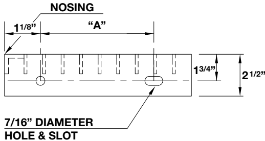
CROSS SECTION: GRATING DEPTH FROM 1-1/2" TO 1-3/4" AND ALL ALUMINUM TREADS
